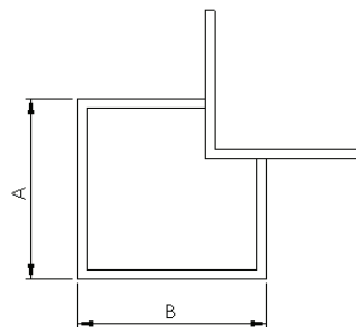
CORNER PROFILE
